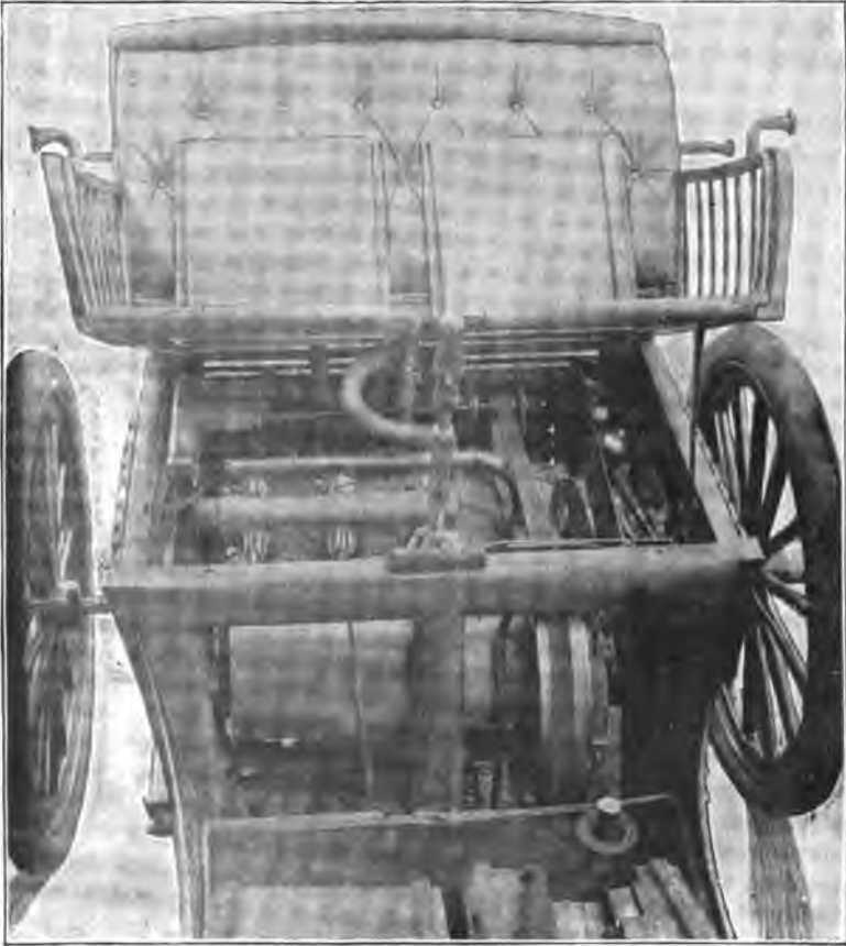
FIG. 389. —View of the Motor and General Mechanism of a Duryea Carriage, giving an idea of the ready accessibility of the parts. The single lever for combining the three functions of steering, throwing on the clutch and throttling the engine is shown rising to the front of the seat.
